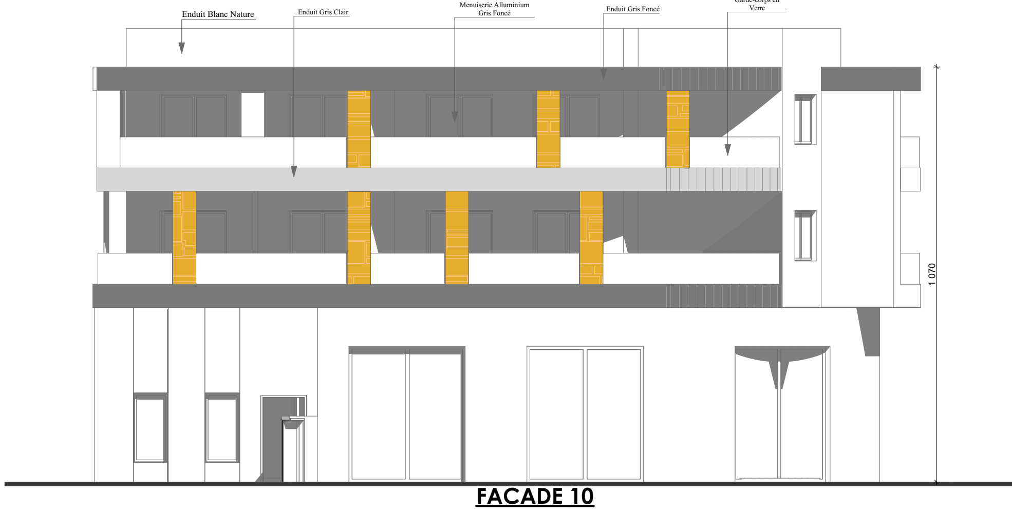
FACADE 10
