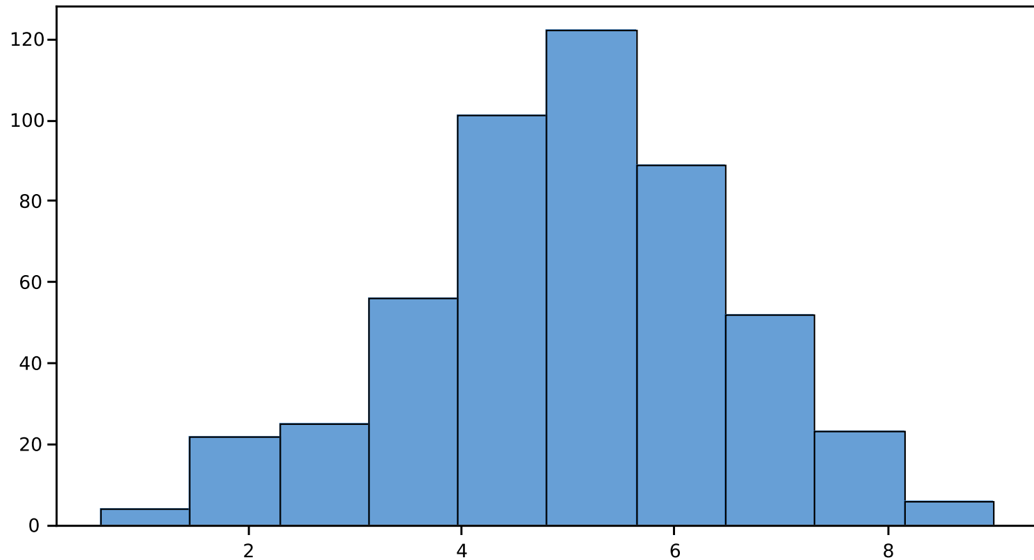
Basic Histogram
