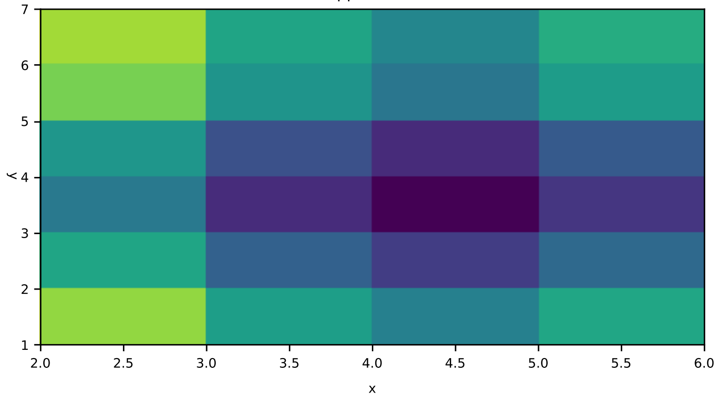
Clipped Imshow
