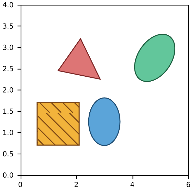
Patch Primitives
