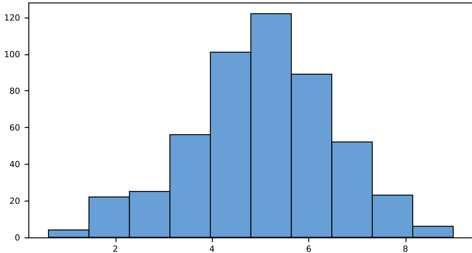
Basic Histogram
