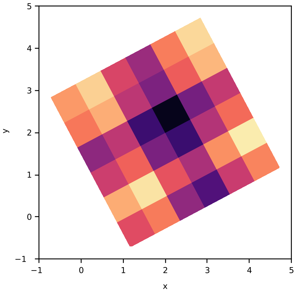
Transformed Imshow
