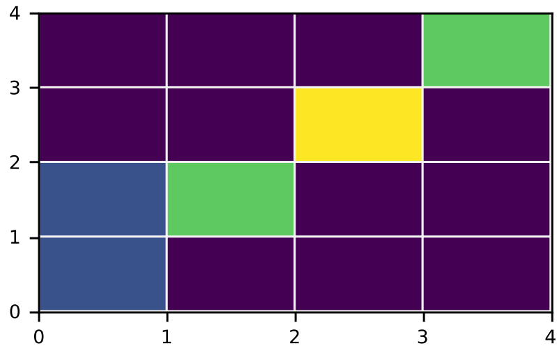
Hist2D
