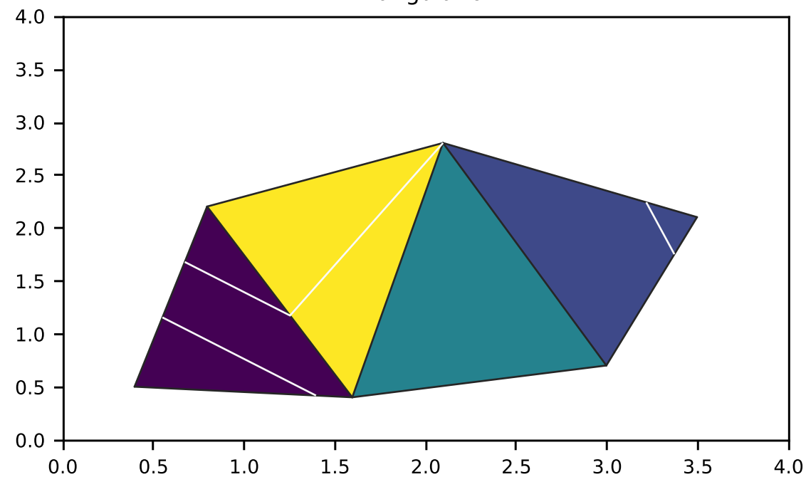
Triangulation
