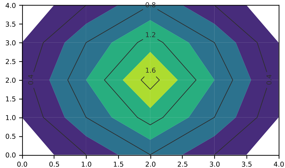
Contour + Contourf
