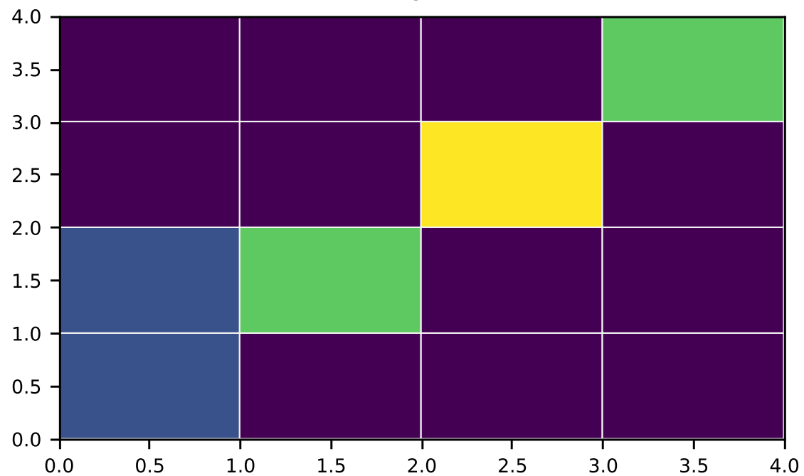
Hist2D
