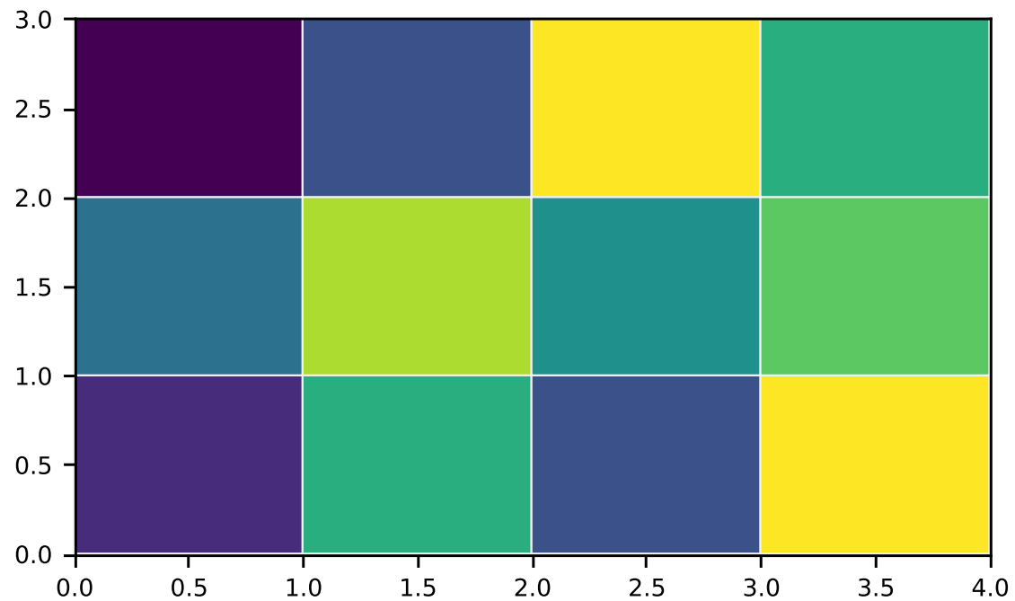
PColorMesh
