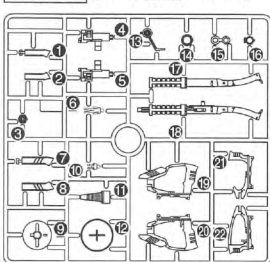
Pパーツ (ABS樹脂: ABS)
