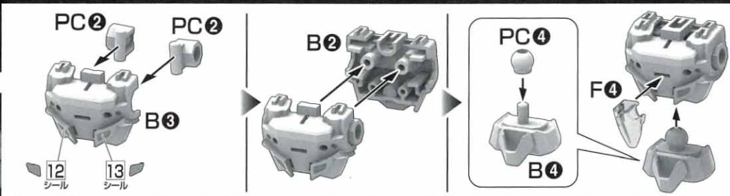
BODY UNIT
