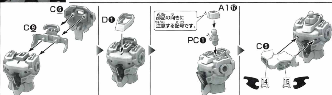
BODY UNIT
