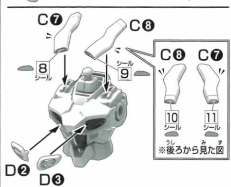
WAIST UNIT
