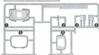
A1パーツ(ホワイト) (PS) A1 Parts (White)
