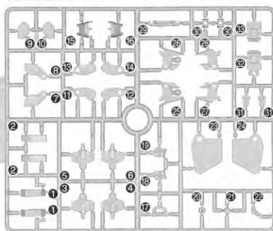
Cパーツ (ABS樹脂: ABS)
