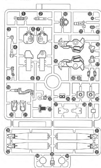
Gパーツ (×2) (ABS樹脂: ABS)
