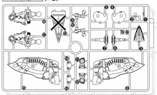
Fパーツ(グレー) (PS) F Parts (Gray) (×2)
