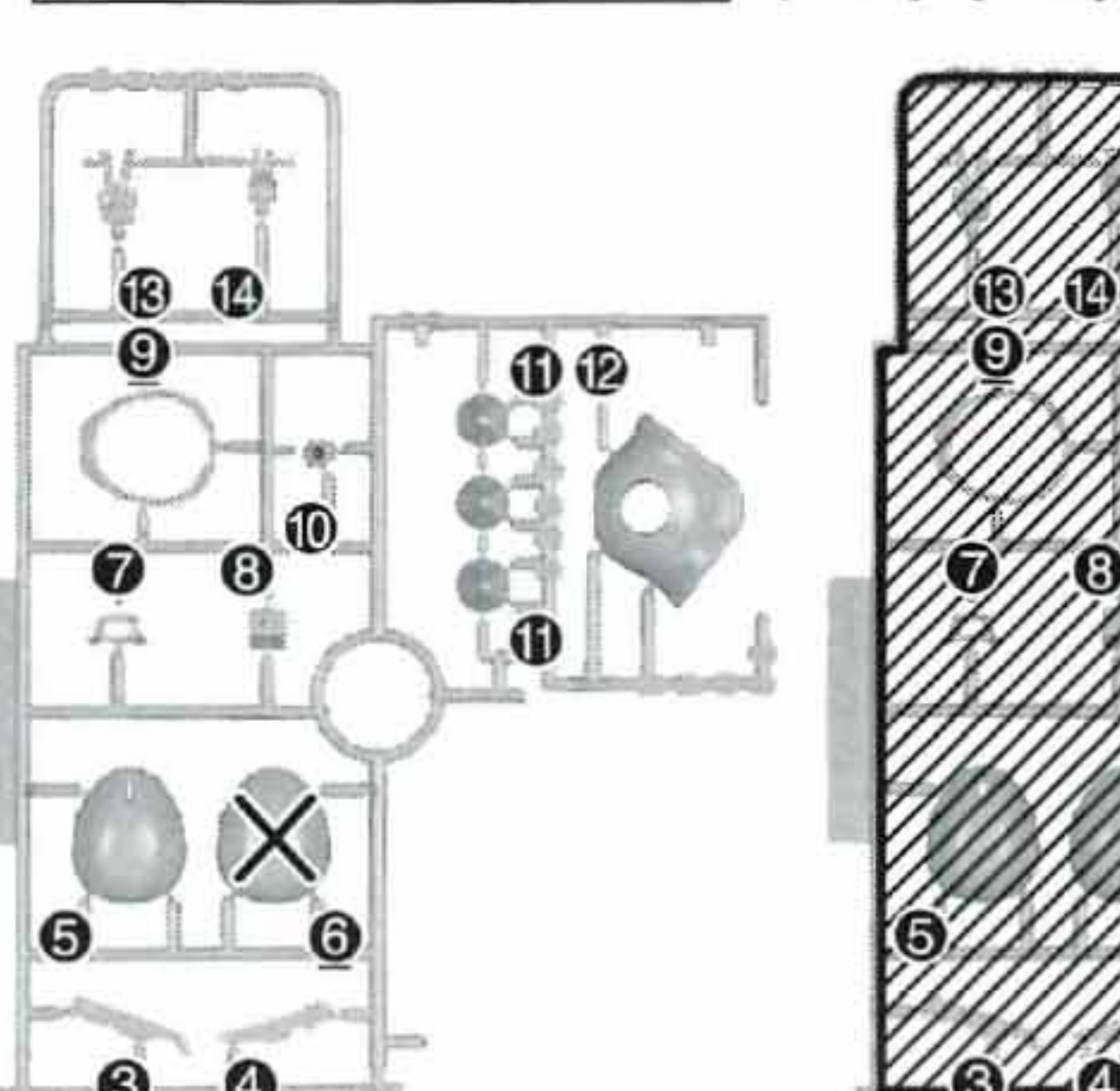
Bパーツ(ホワイト) B Parts (White) (×2) (PS)
