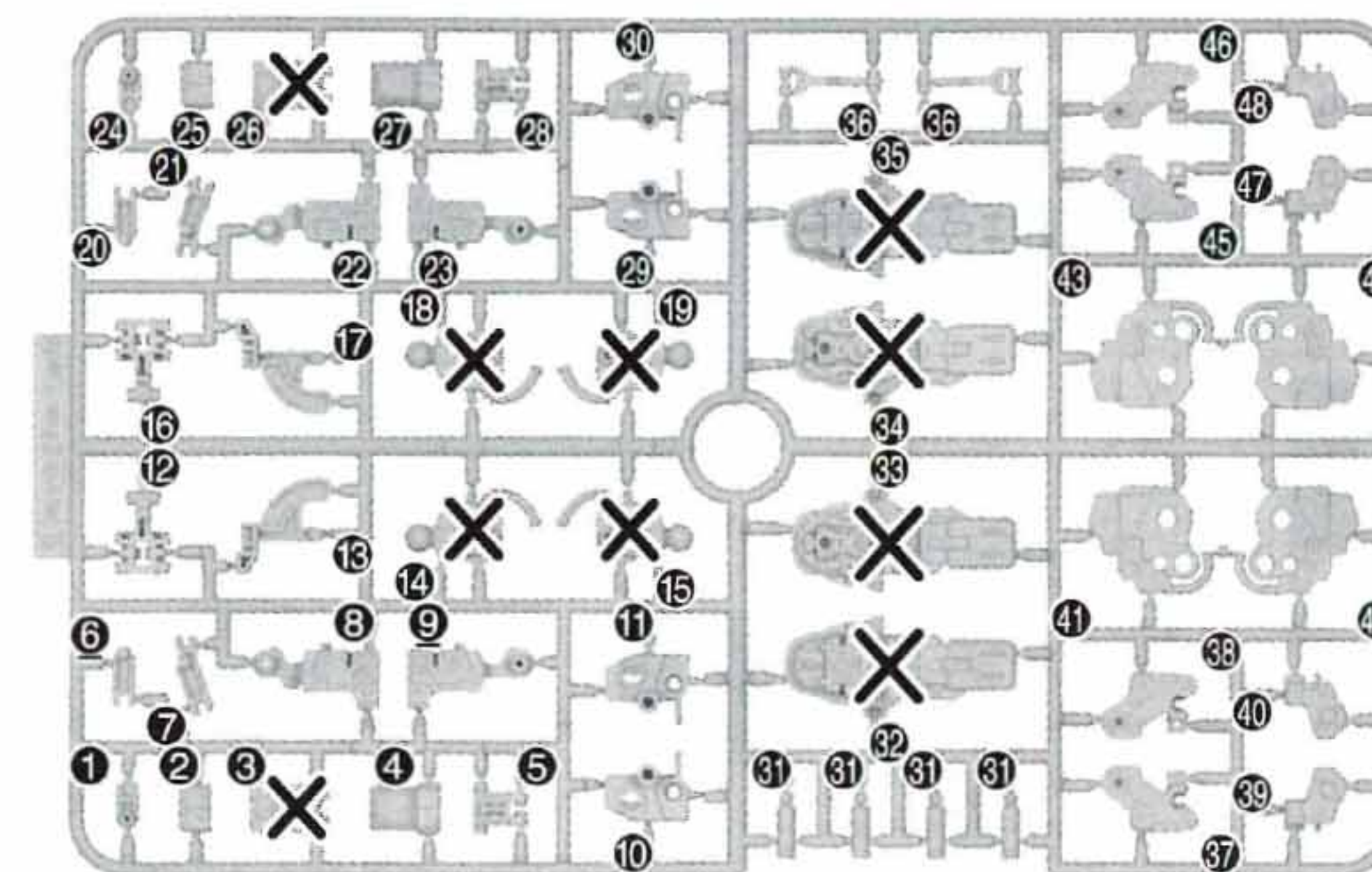
H2パーツ(レッド) H2 Parts (Red) (PS)
