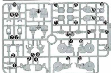
Fパーツ(グレー) (ABS) F Parts (Gray)
