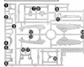
Tパーツ(イロバラ) (PS) T Parts (Multi-colored)
