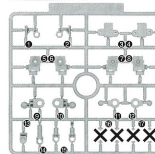
Hパーツ(グレー) (ABS) H Parts (Gray)
