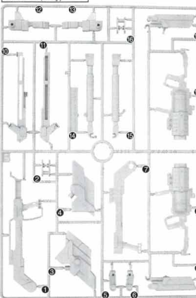
J1パーツ(グレー) (PS) J1 Parts (Gray)
