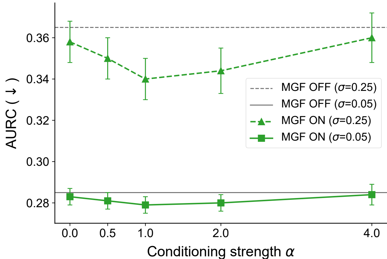
AURC vs \alpha under Gaussian noise (min \sigma = 0.05 , max \sigma = 0.25 )
