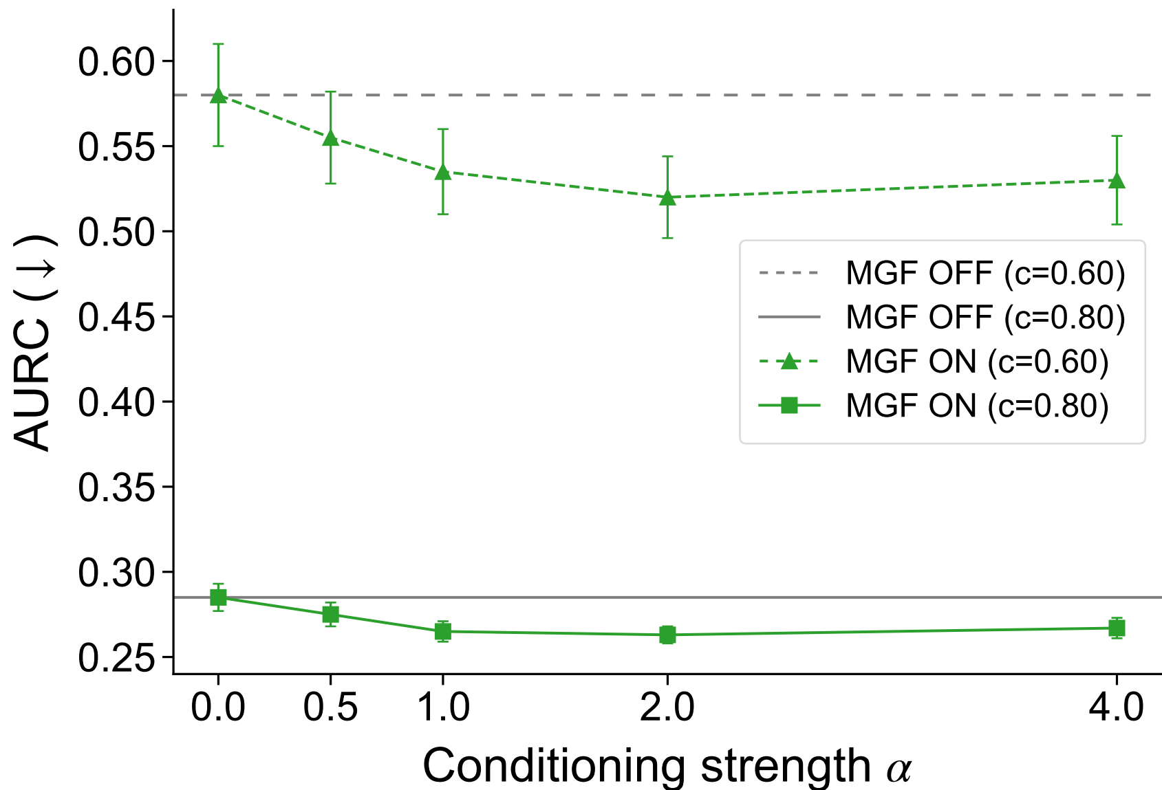
AURC vs \alpha under contrast shift ( c \in [0.60, 0.80] ; lower = more severe)
