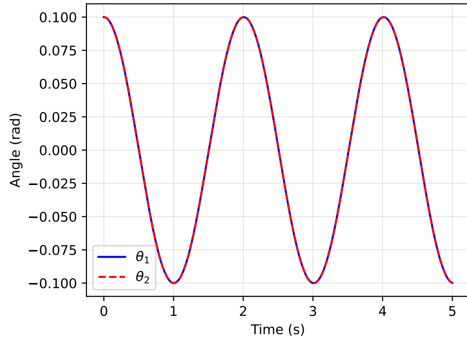
Symmetric Mode
