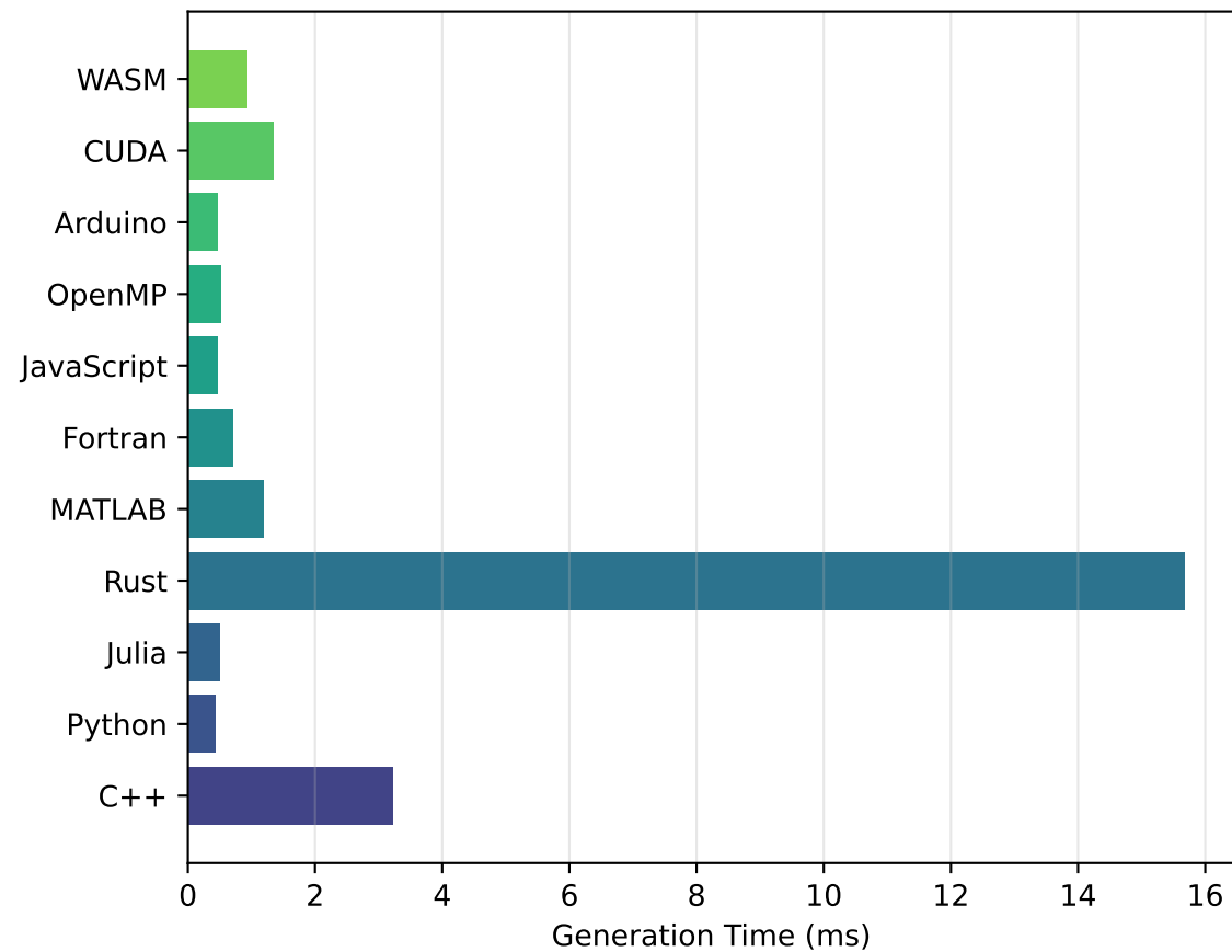
Code Generation Time
