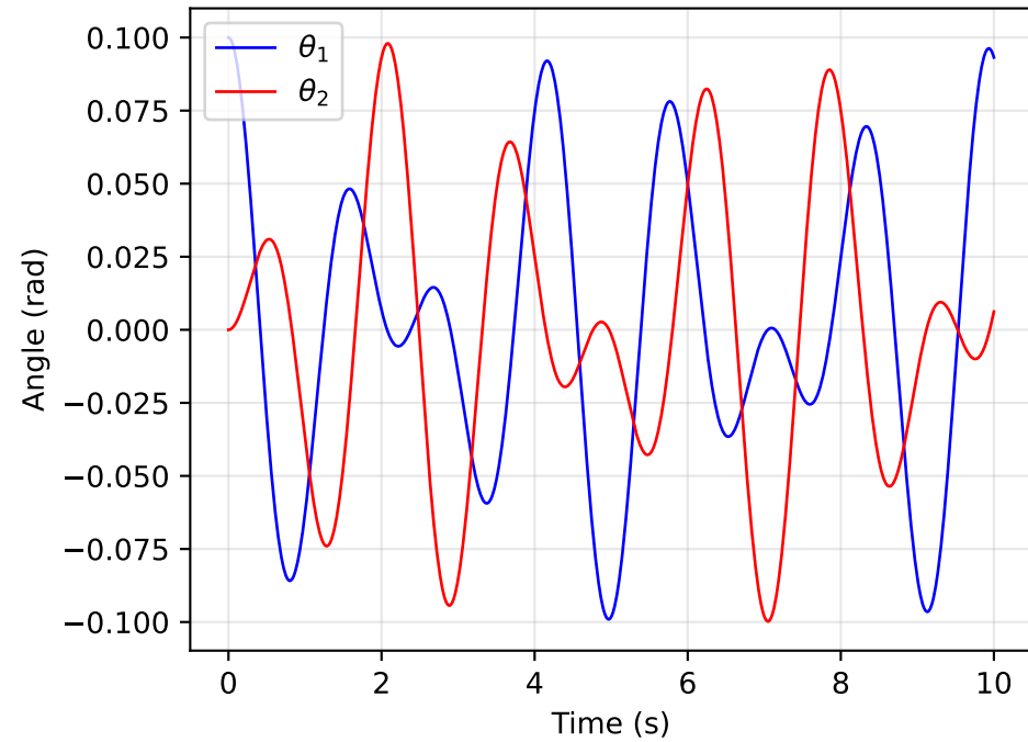
Beating Phenomenon
