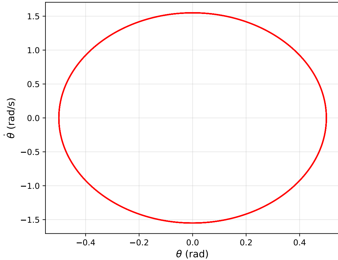
Phase Portrait
