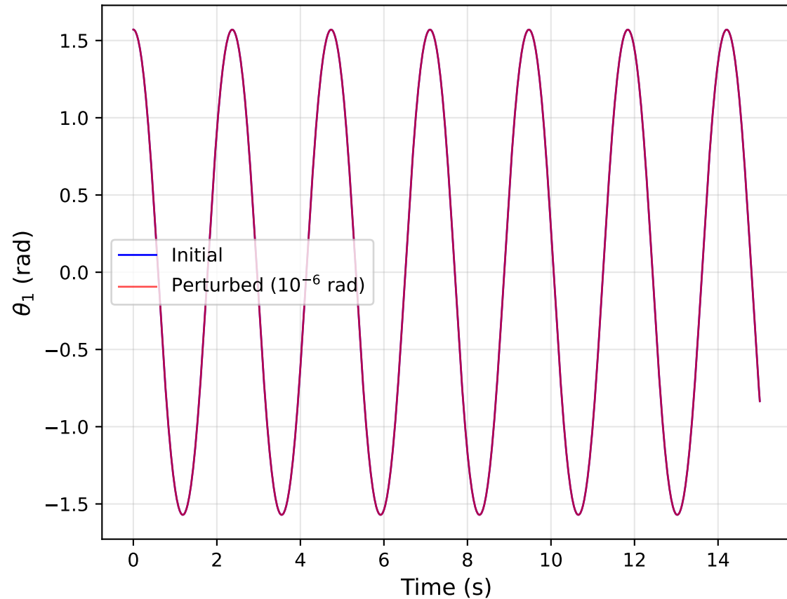
Sensitive Dependence on Initial Conditions
