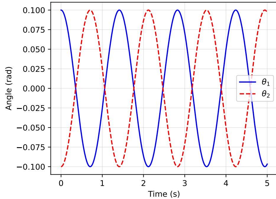
Antisymmetric Mode
