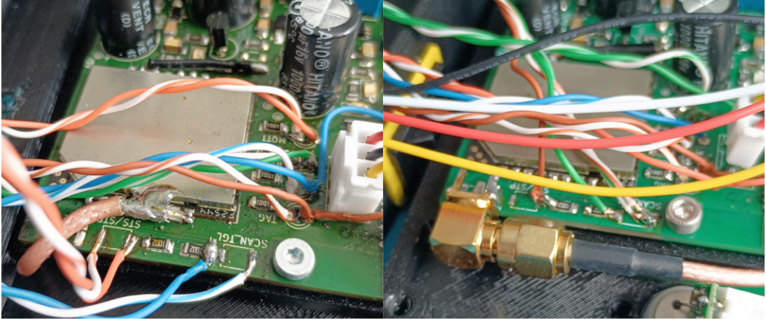
Figure 5: Antenna connection comparison
