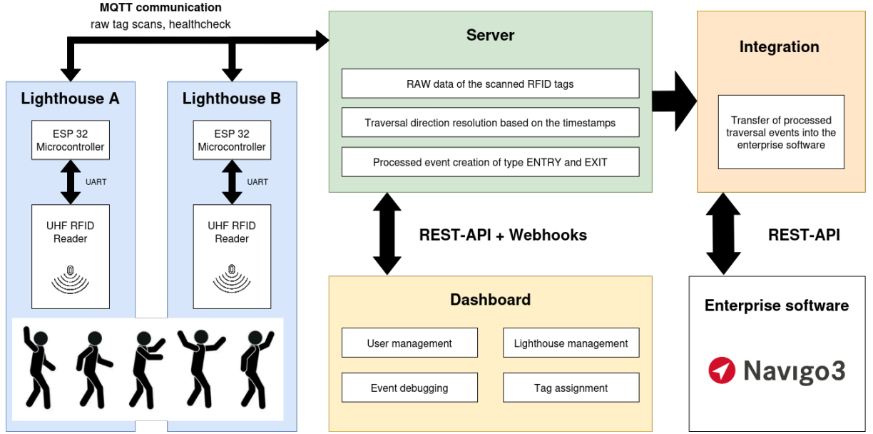
Figure 1: System architecture block diagram
