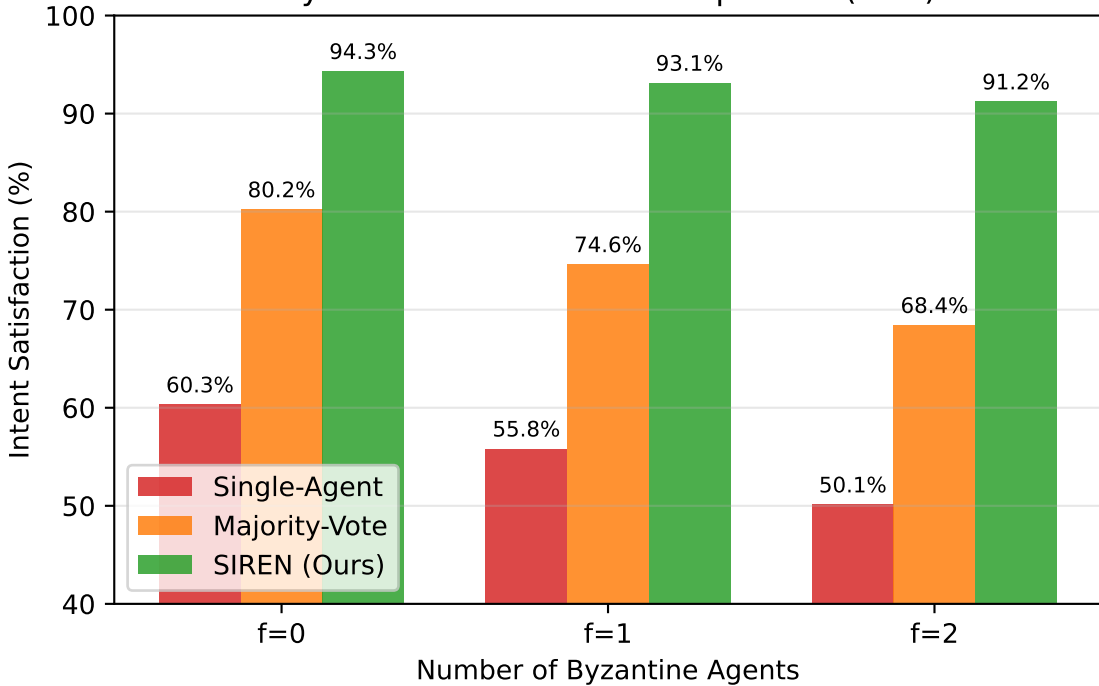
Byzantine Robustness Comparison (n=7)
