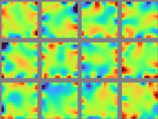
classic decoding
