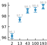
HCP-YA Task21
