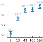
HCP-YA Task21
