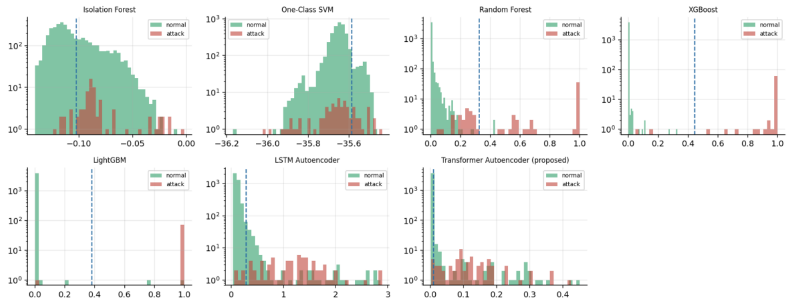
score_dists Score distributions + threshold — test
