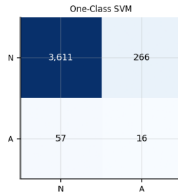
confusion_grid Confusion matrices — held-out test
