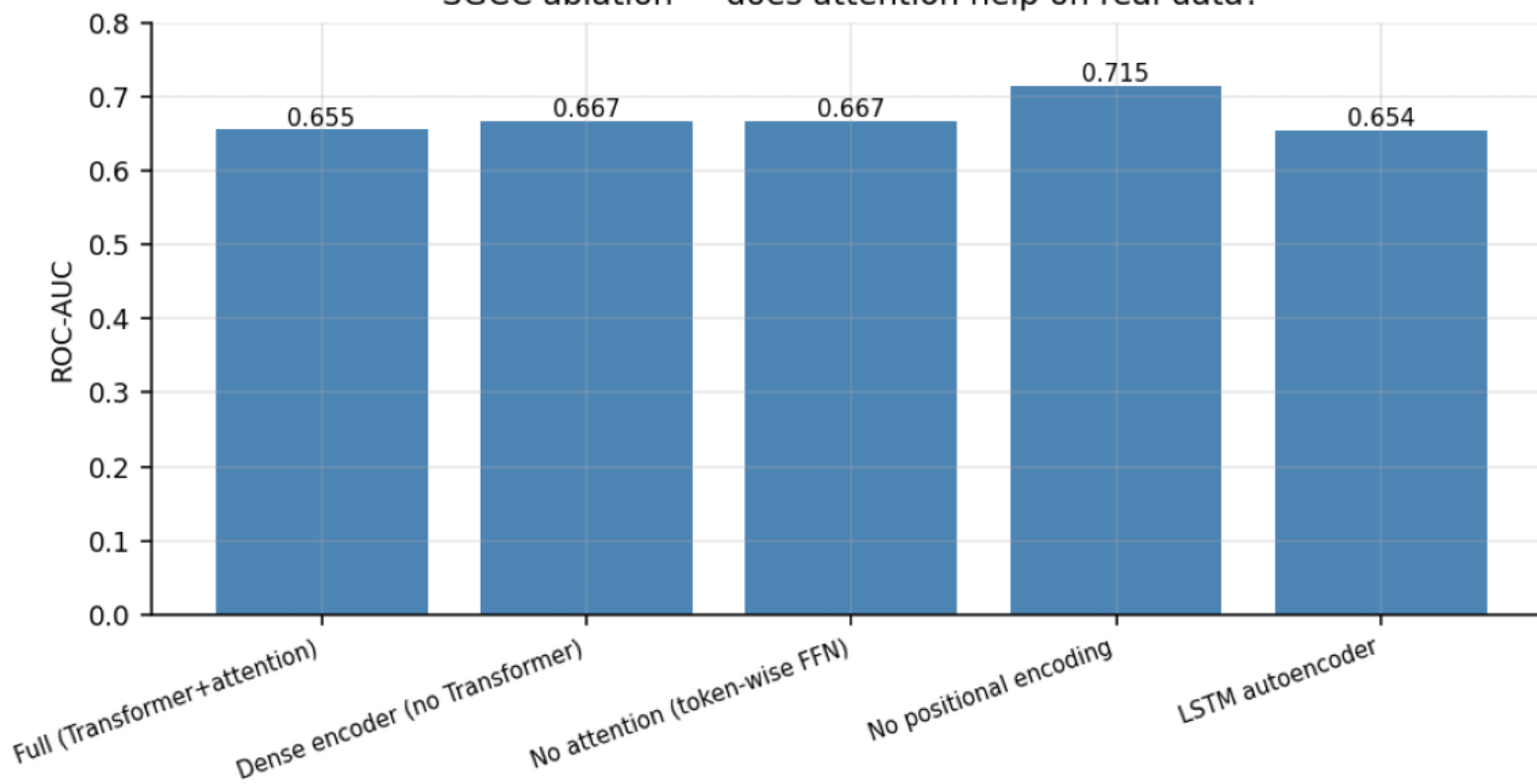
SGCC ablation — does attention help on real data?
