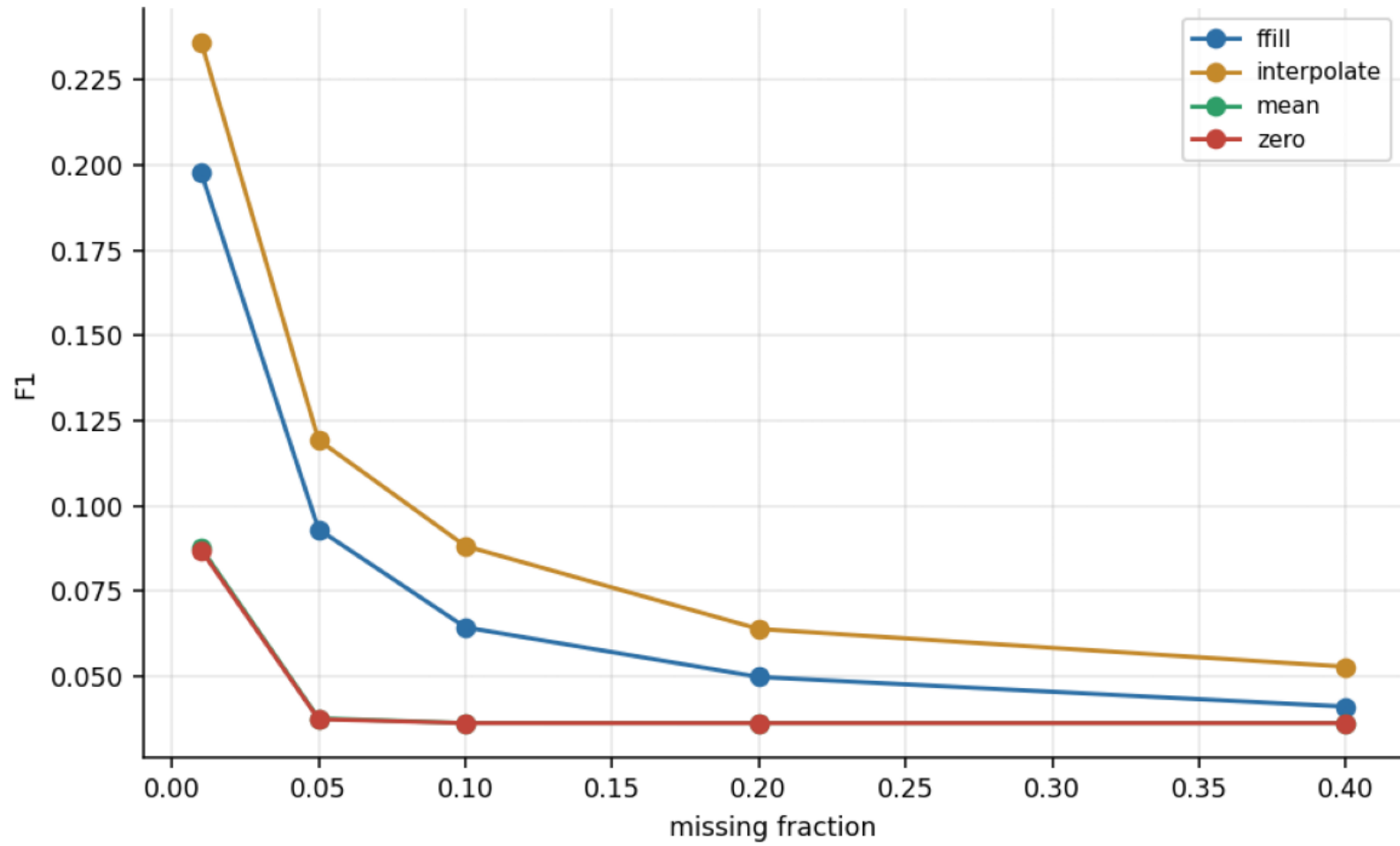
Missing-data robustness by imputation strategy
