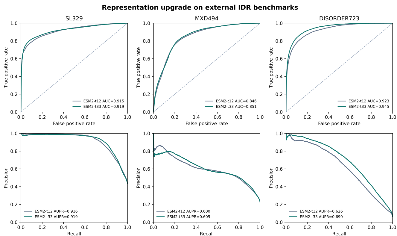
Figure 3 ROC and precision-recall curves for the ESM2-t12 to ESM2-t33 representation upgrade. The largest and statistically supported AUC gain occurs on DISORDER723.
