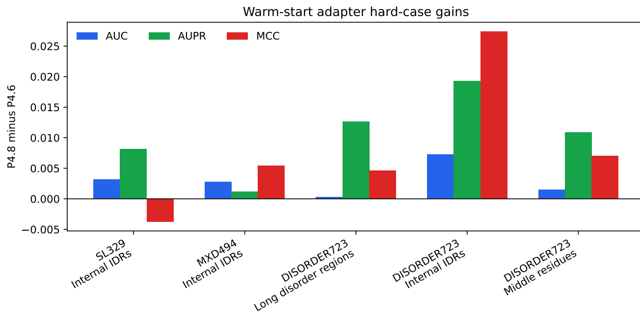
Figure 4 Hard-case gains for the P4.8 warm-start RegionAdapterMoETCN ensemble relative to the P4.6 ESM2-t33 RegionAwareTCN ensemble. The largest practical improvement occurs on DISORDER723 internal IDRs.
