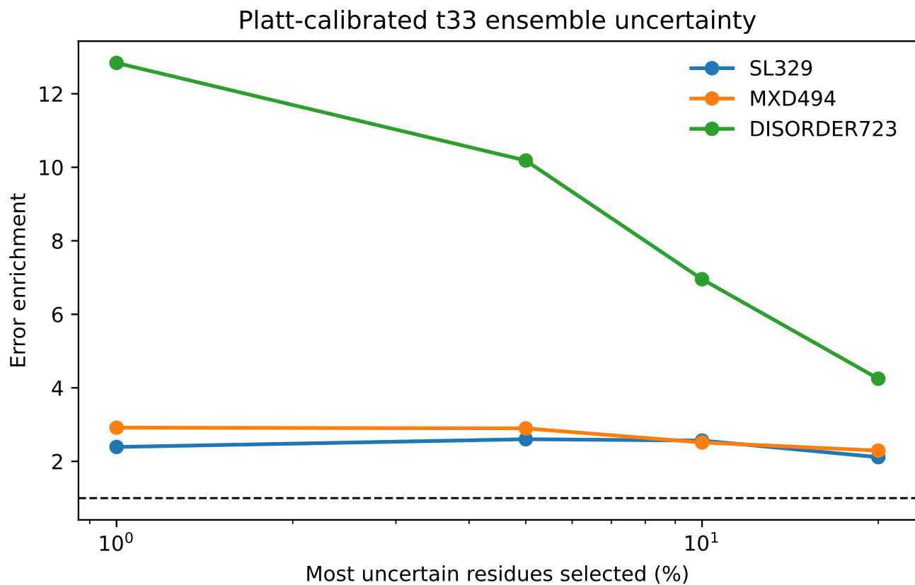
Figure 6 Platt calibration and uncertainty-error enrichment. Calibrated uncertainty identifies error-enriched residues, especially on the highly imbalanced DISORDER723 benchmark.
