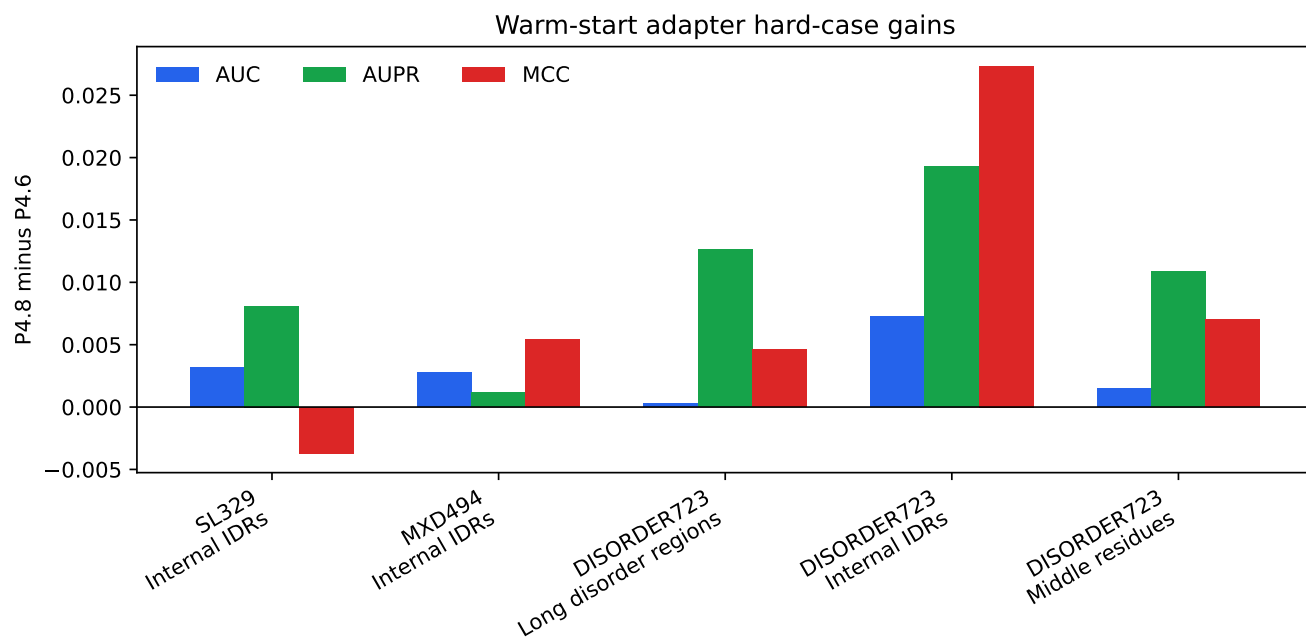
Figure 5 Hard-case gains for the P4.8 warm-start RegionAdapterMoETCN ensemble relative to the P4.6 ESM2-t33 RegionAwareTCN ensemble. The largest practical improvement occurs on DISORDER723 internal IDRs.
