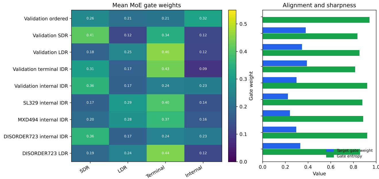
Figure 7 Exploratory MoE gate specialization analysis. Gate weights are partially aligned with validation SDR and terminal-IDR strata but are not clean one-hot biological region assignments; routing is therefore interpreted as an auxiliary score-specialization mechanism.
