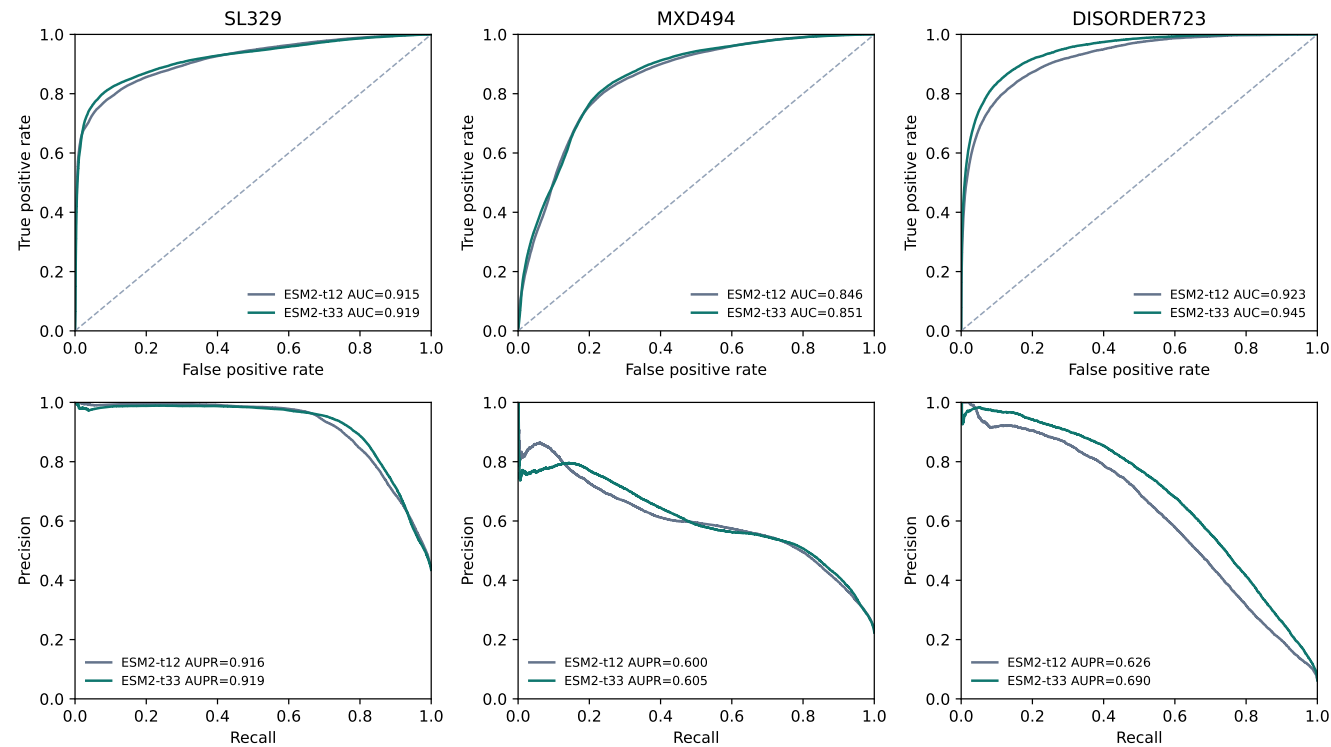
Figure 4 ROC and precision-recall curves for the ESM2-t12 to ESM2-t33 representation upgrade. The largest and statistically supported AUC gain occurs on DISORDER723.
