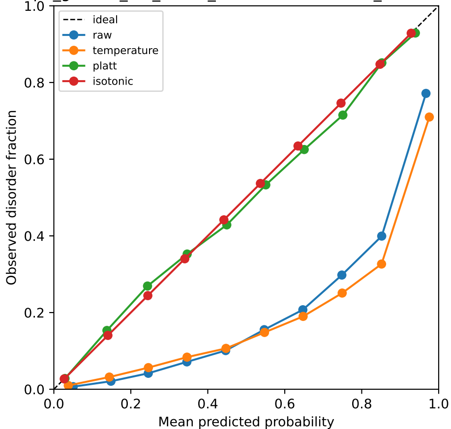
p2_generic_tcn_3seed_ensemble / DM1229_Validation
