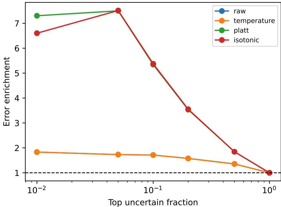
p2_generic_tcn_3seed_ensemble / DM1229_Validation
