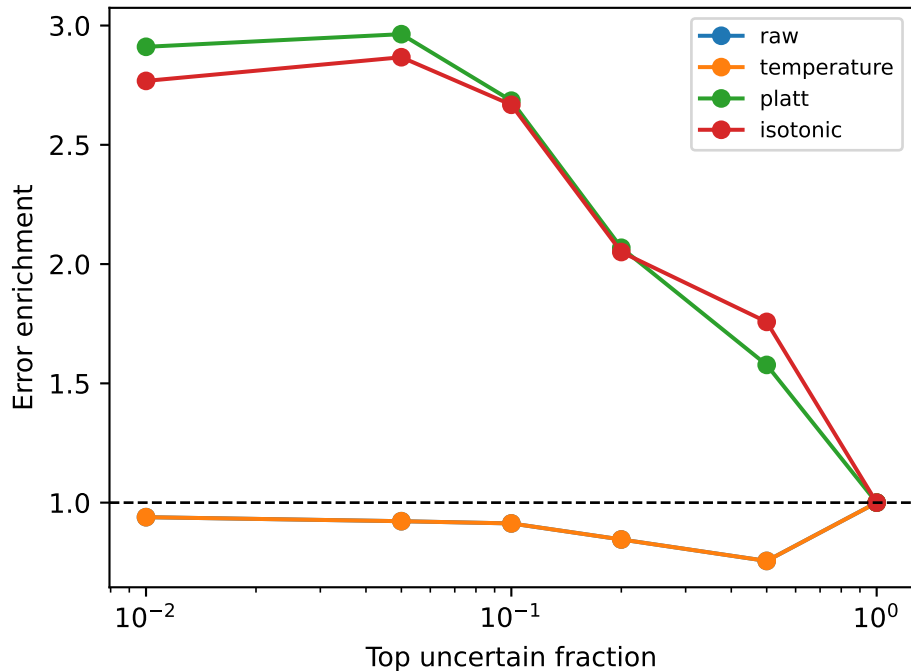
p2_generic_tcn_3seed_ensemble / MXD494
