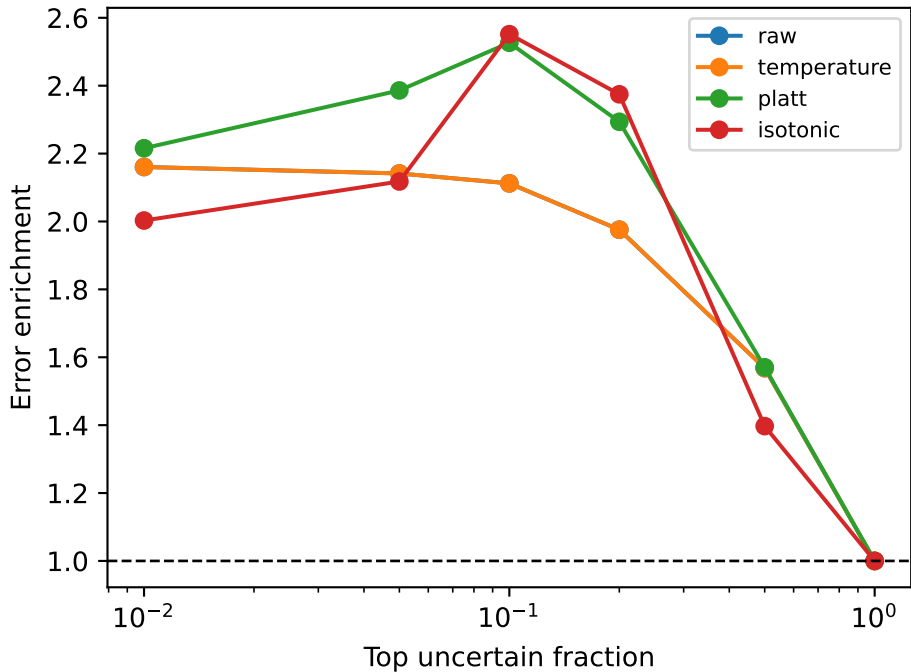
p2_generic_tcn_3seed_ensemble / SL329
