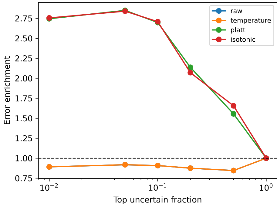
p2_region_aware_tcn_3seed_ensemble / MXD494
