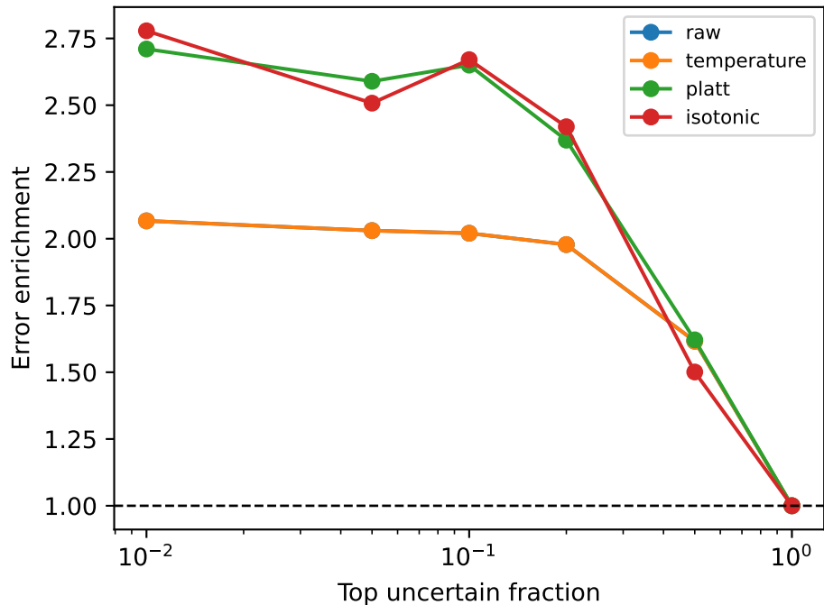
p2_region_aware_tcn_3seed_ensemble / SL329
