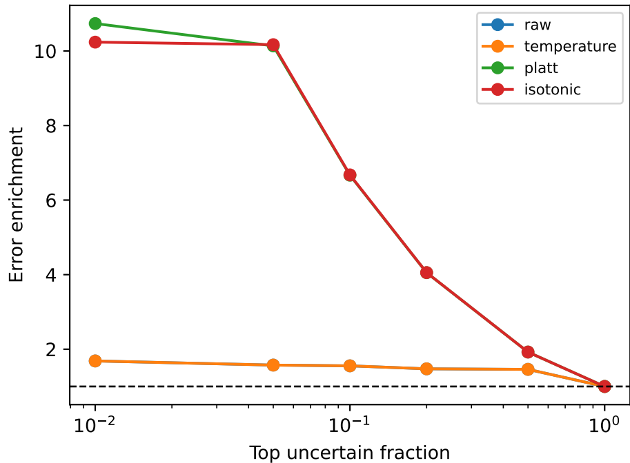
p2_tcn_6model_ensemble / DISORDER723
