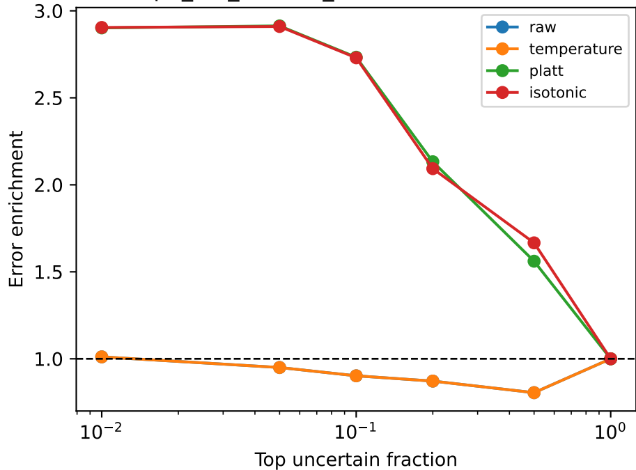
p2_tcn_6model_ensemble / MXD494
