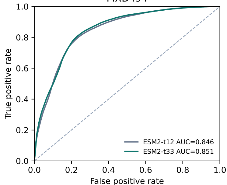
MXD494
