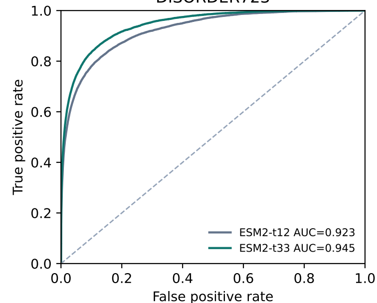
DISORDER723
