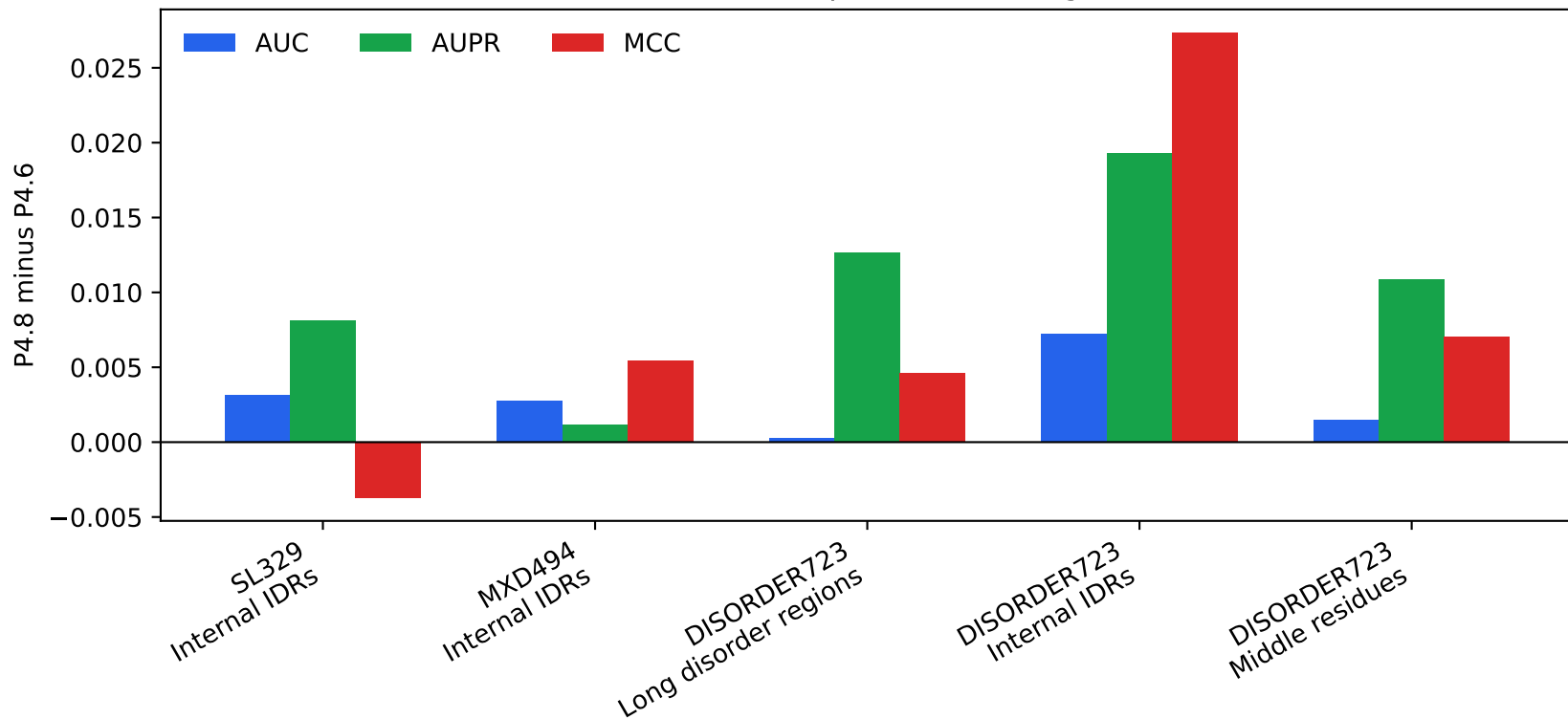
Warm-start adapter hard-case gains
