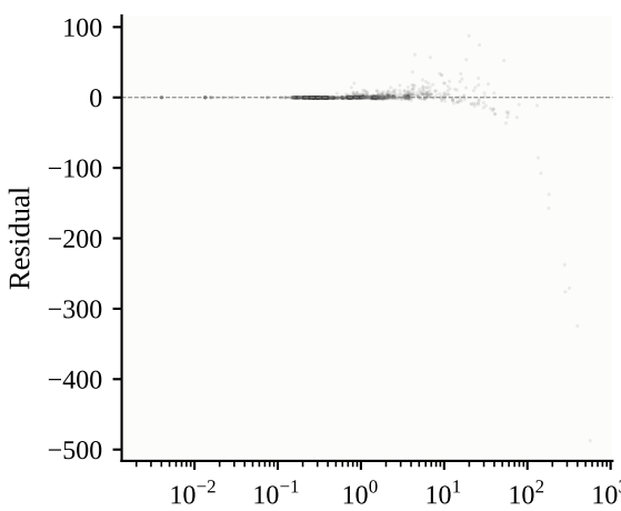
(c) Residual distribution
