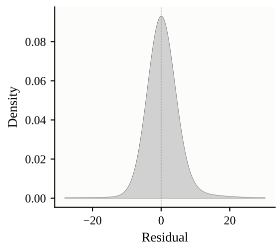
(c) Residual distribution
