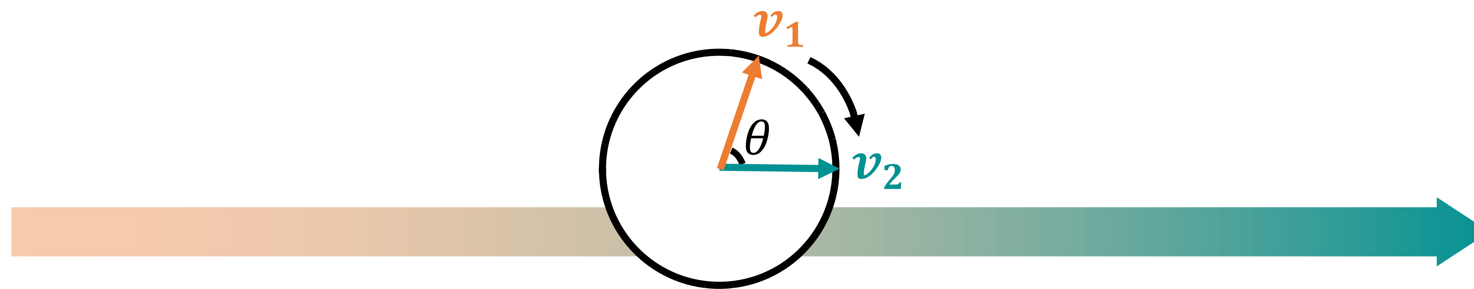
Interpolated styles
