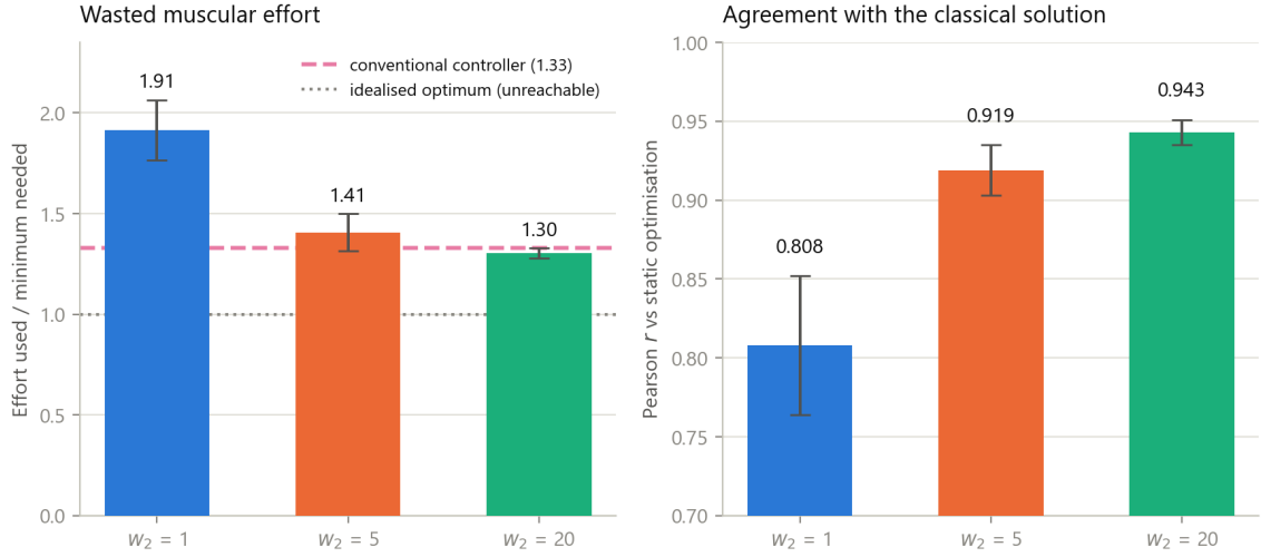
Figure 7.3. Effect of the effort weight, five seeds per setting. Left: muscular effort relative to the classical minimum. The dashed line is the conventional controller’s 1.33; the dotted line is the idealised optimum of 1.00, which section 7.9.3 shows is not attainable in closed loop. Right: agreement with the classical load-sharing solution. Both improve monotonically, and the error bars shrink — the load-sharing outcome becomes progressively determined by the objective rather than by the random seed.
