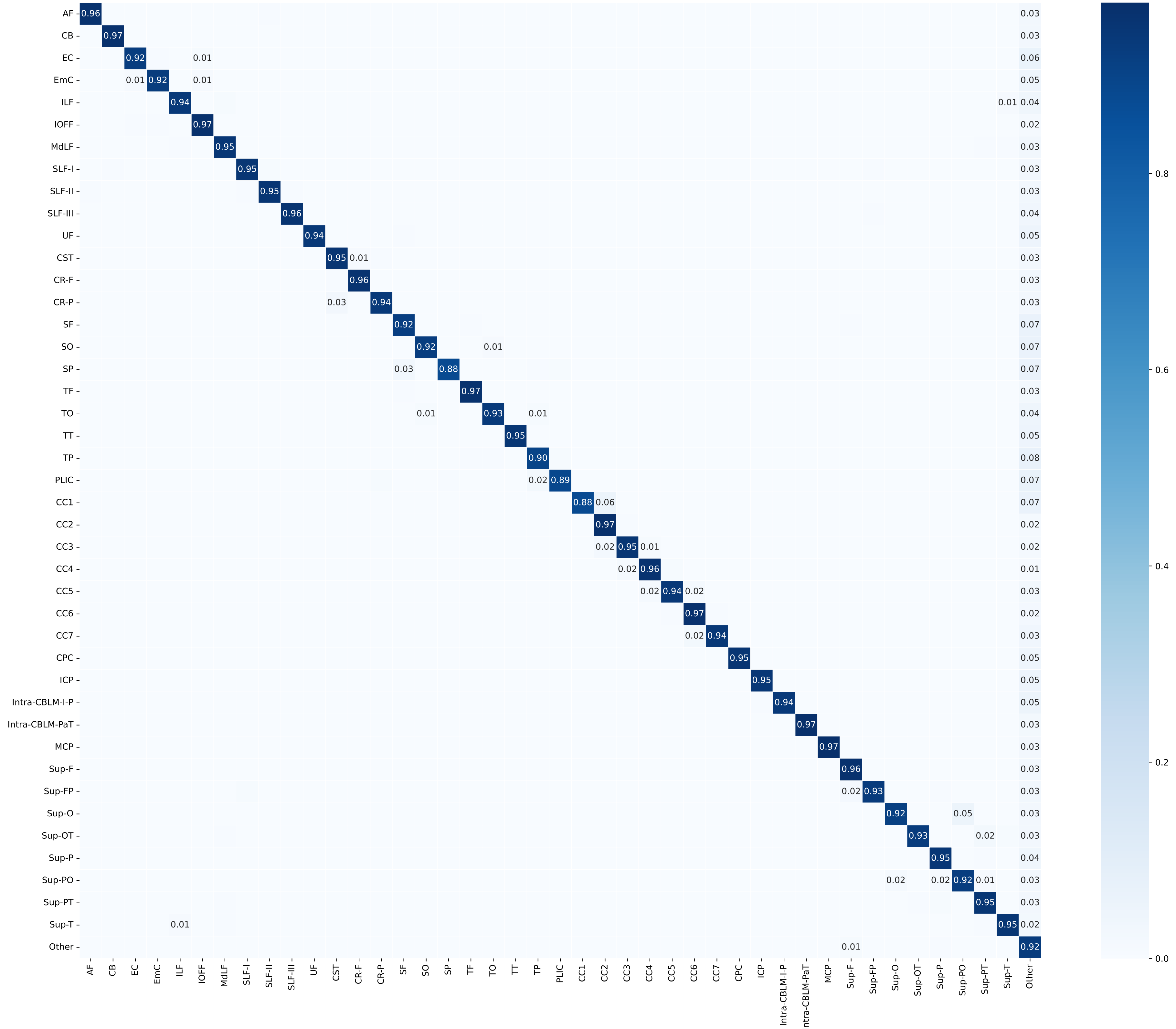
Accuracy: 93.85 %, Macro F1: 92.41, Prediction duration: 5.44 s for 6200000 Streamlines
