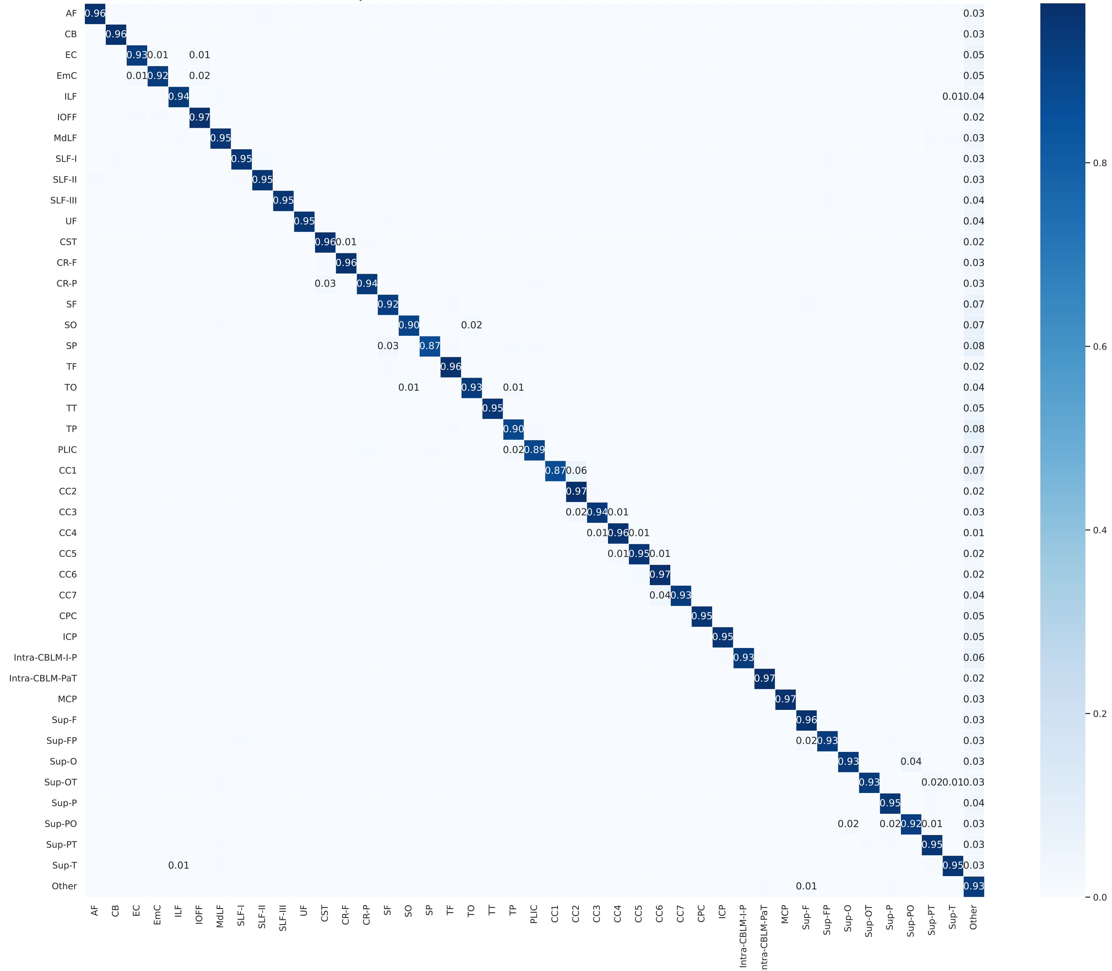
Confusion Matrix for all Subjects Accuracy: 93.91 %, Macro F1: 92.49, Prediction duration: 4.65 s for 6200000 Streamlines
