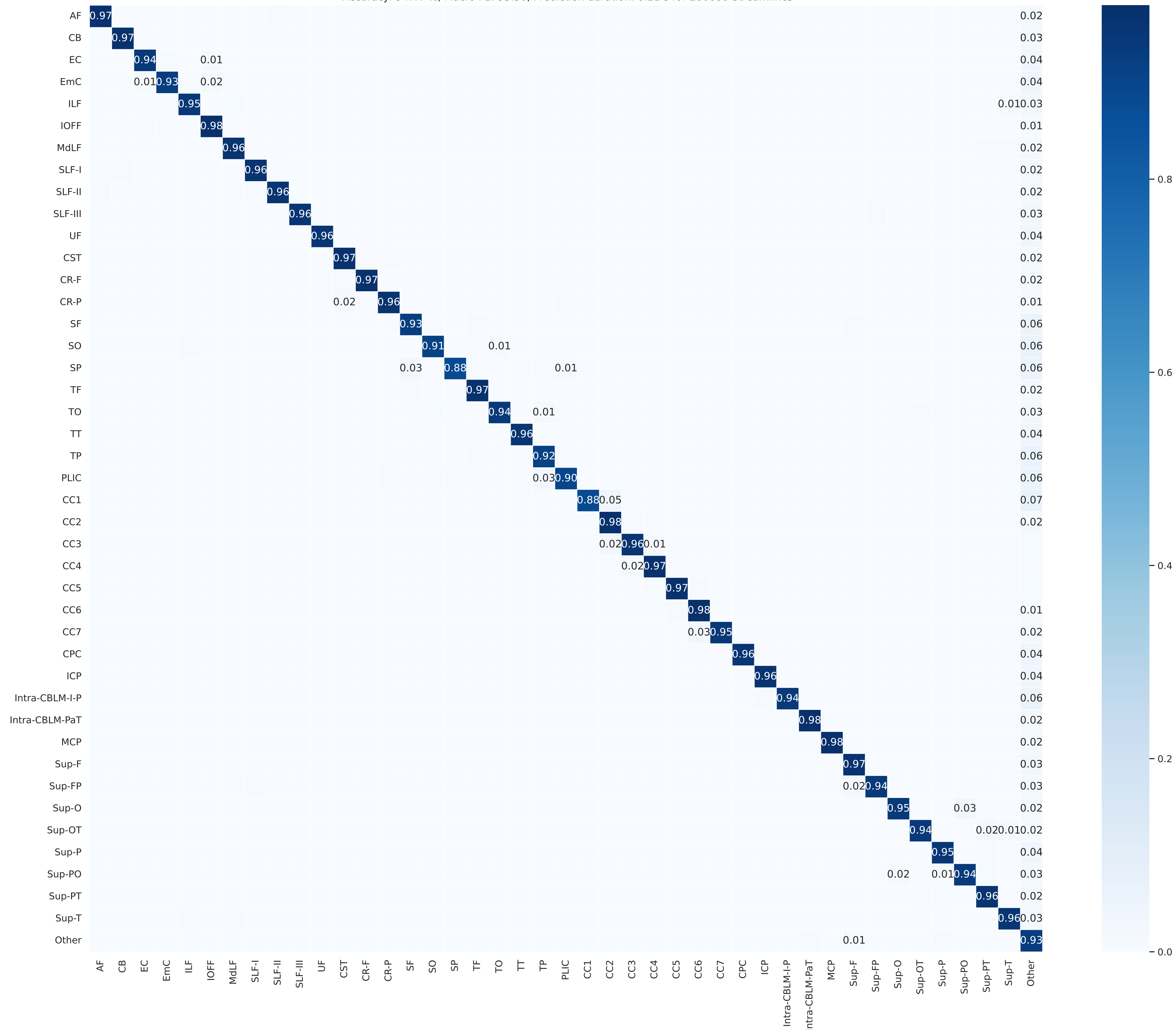
Accuracy: 94.47 %, Macro F1: 93.30, Prediction duration: 0.21 s for 200000 Streamlines
