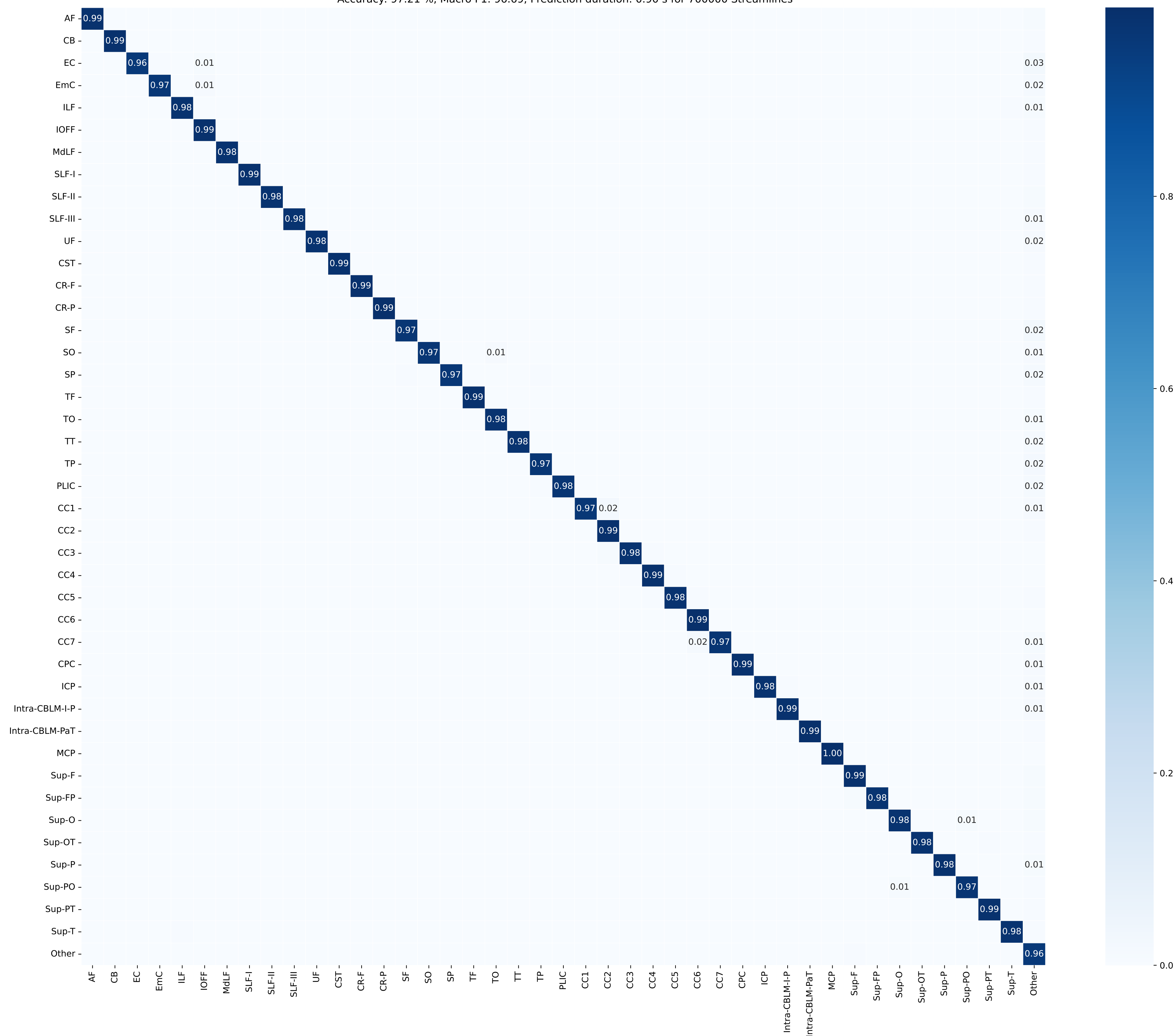
Confusion Matrix for all Subjects Accuracy: 97.21 %, Macro F1: 96.69, Prediction duration: 0.90 s for 700000 Streamlines
