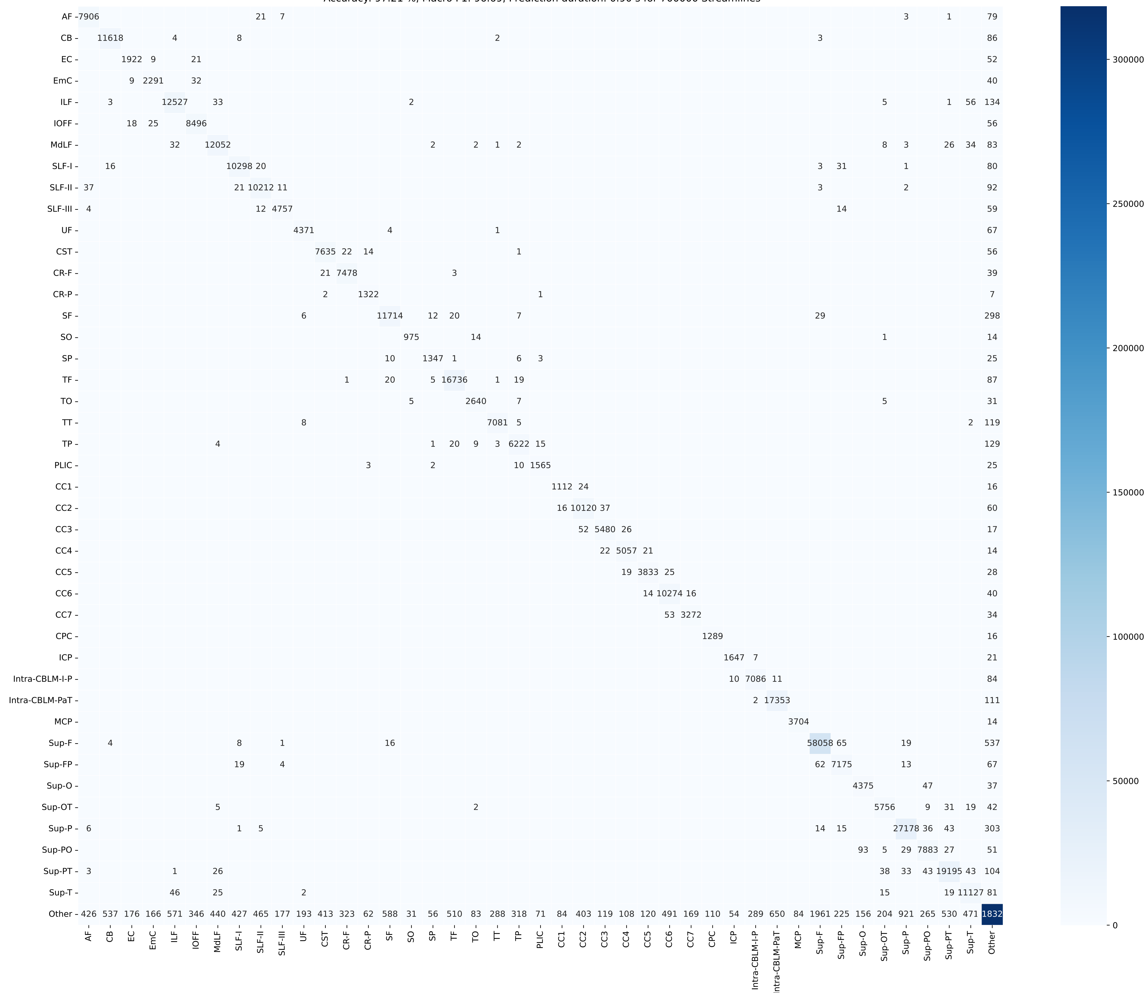
Unnormalized Confusion Matrix for all Subjects Accuracy: 97.21 %, Macro F1: 96.69, Prediction duration: 0.90 s for 700000 Streamlines
